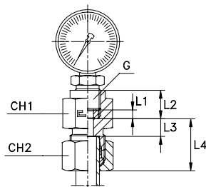
Type: 1059.. B3 Ring Metal washer seal
